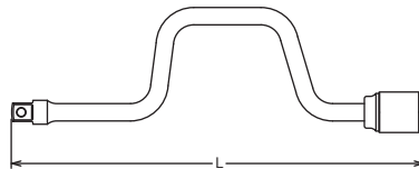
4781N-450 Flexible Speed Handle Gelenkgriff-Winde Vilebrequin
